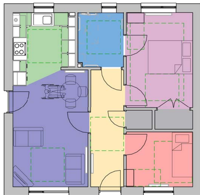
House Type Q02 - Ground Floor 1:100
