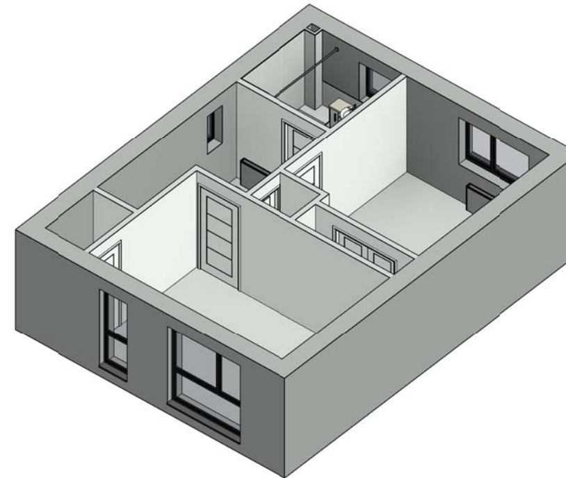
House Type A01 - First Floor 3D View
