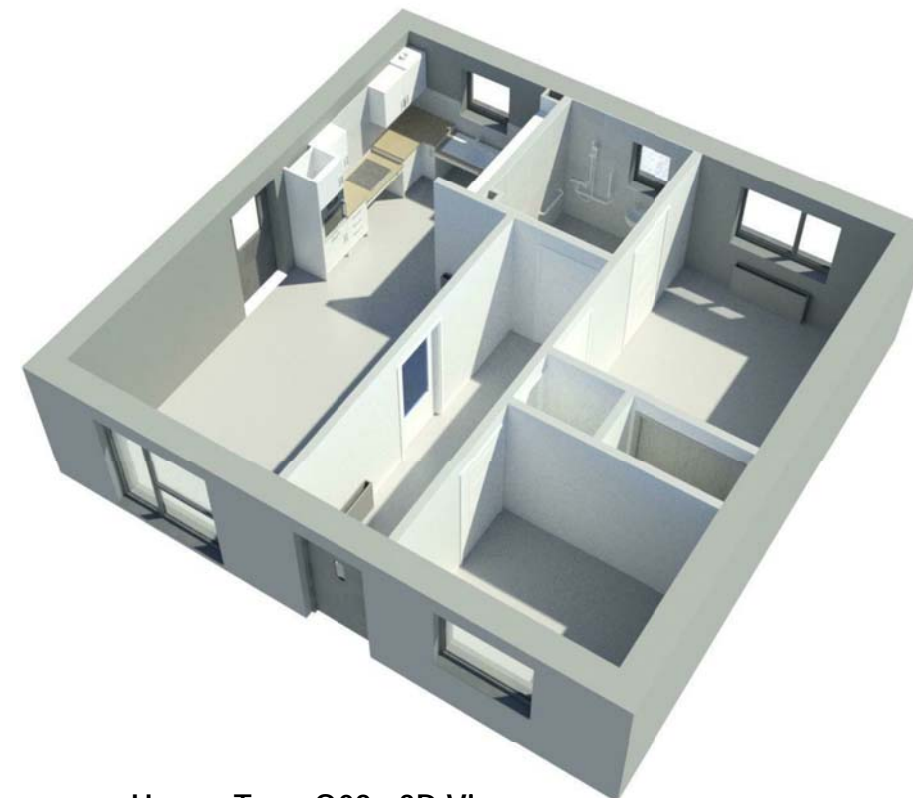
House Type Q02 - 3D View
