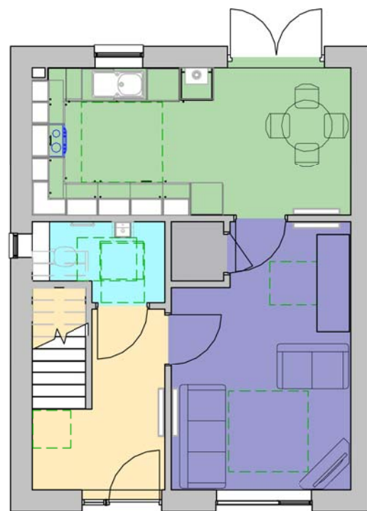
House Type A01 - Ground Floor 1:100
