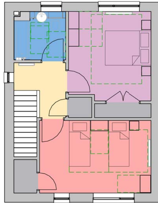
House Type A01 - First Floor 1:100
