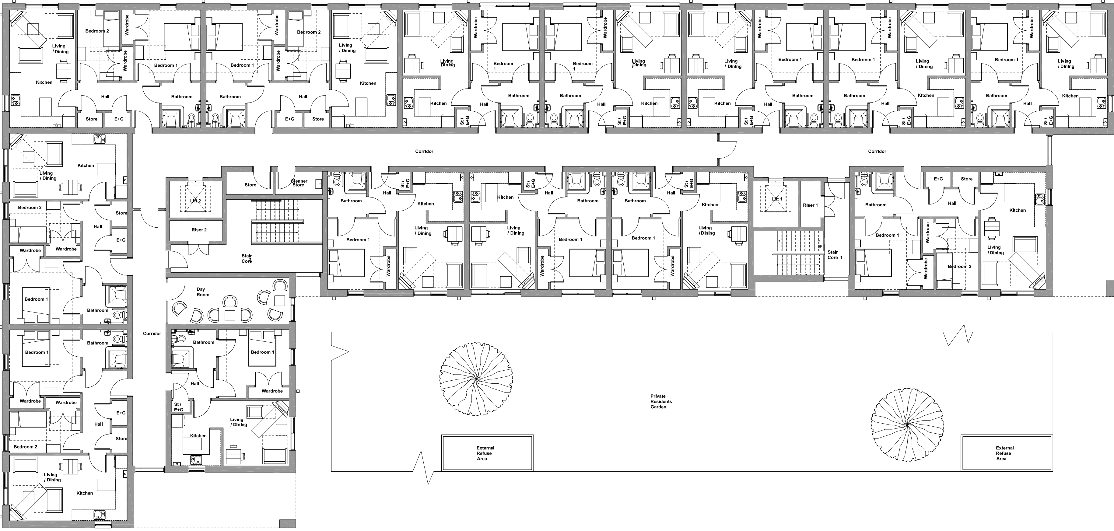
Ground Floor 8 Sheltered Housing Unit Quantity: 14No. 1 Bed Flat & 10No. 2 Bed Flat
