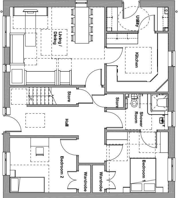
4B6P 6 Wheelchair Liveable House Quantity: 1No.
