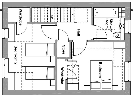
2B4P 3 General Needs House Type A Quantity: 15No.
