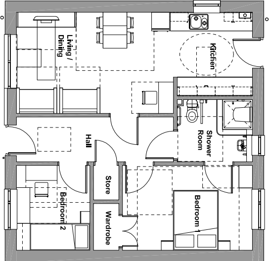
2B3P 1 Amenity Bungalow Quantity: 2No.
