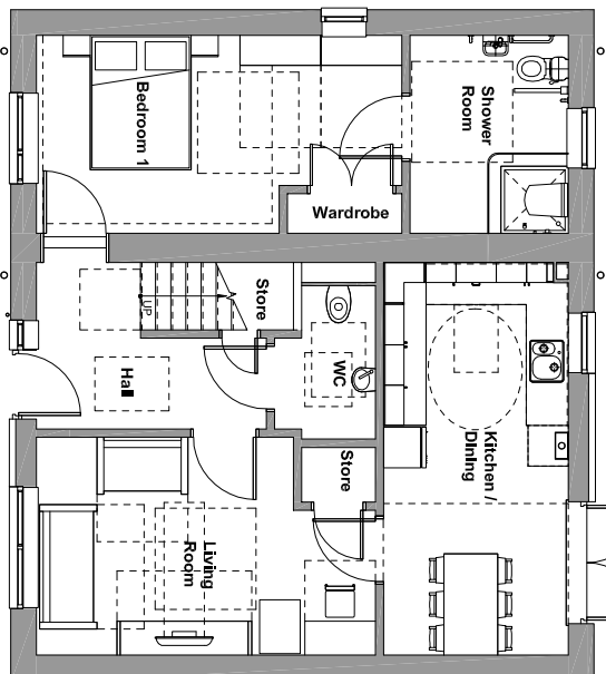
3B5P 5 Wheelchair Liveable House Quantity: 5No.
