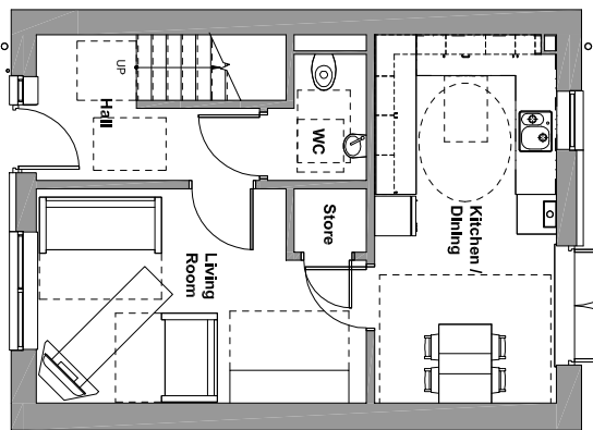
2B4P 3 General Needs House Type A Quantity: 15No.
