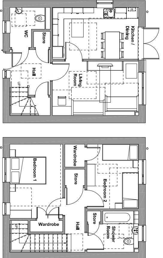
2B4P 4 General Needs House Type B Quantity: 19No.
